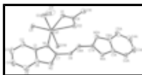
Fig. 1. The asymmetric unit of the title complex. Displacement ellipsoids are drawn at the 30% probability level. H atoms have been omitted for clarity. [Symmetry codes: (A) -x+1, -y+2, -z+1 ; (B) -x+1, -y+2, -z+2 .]
